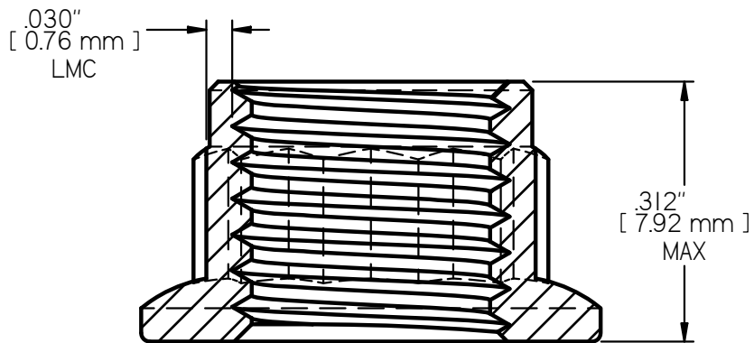
SECTION A-A 5X SCALE
