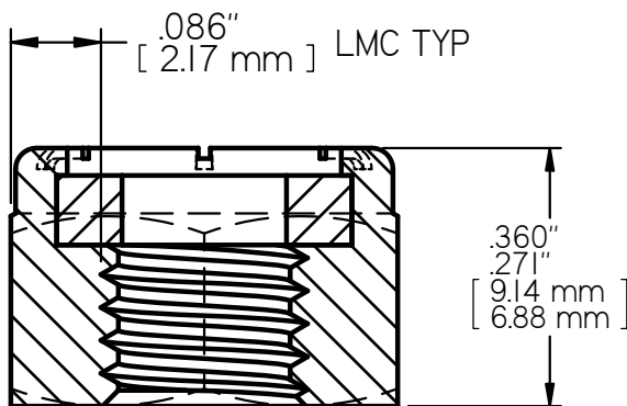
SECTION A-A 4X SCALE
