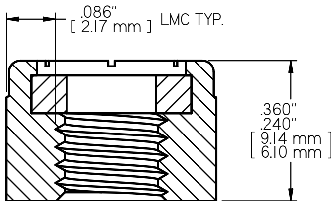
SECTION A-A 5X SCALE
