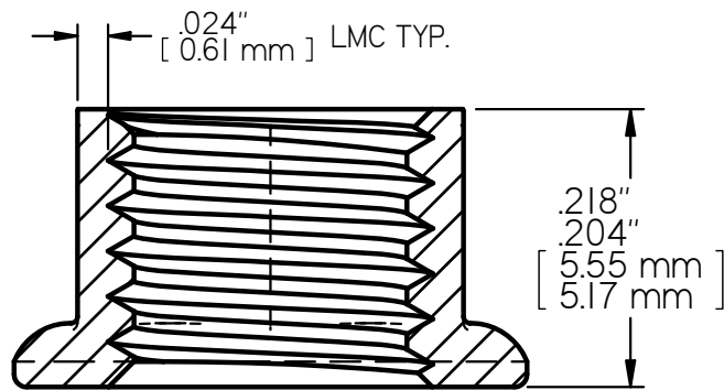
SECTION A-A 6X SCALE
